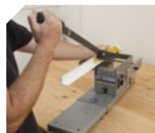
Fast and clean cutting without any risk. No dust nor static PVC chips.
