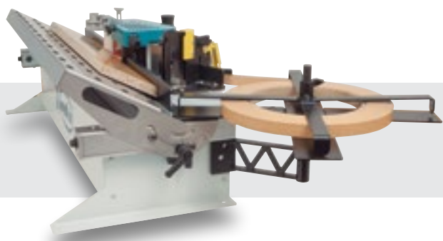
MI250 Tilting table. For gluing panels with a lean from 15° to 50°.
